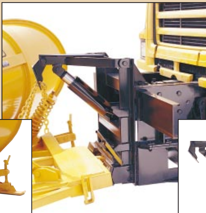
Falls #44B Hitch System Shown
